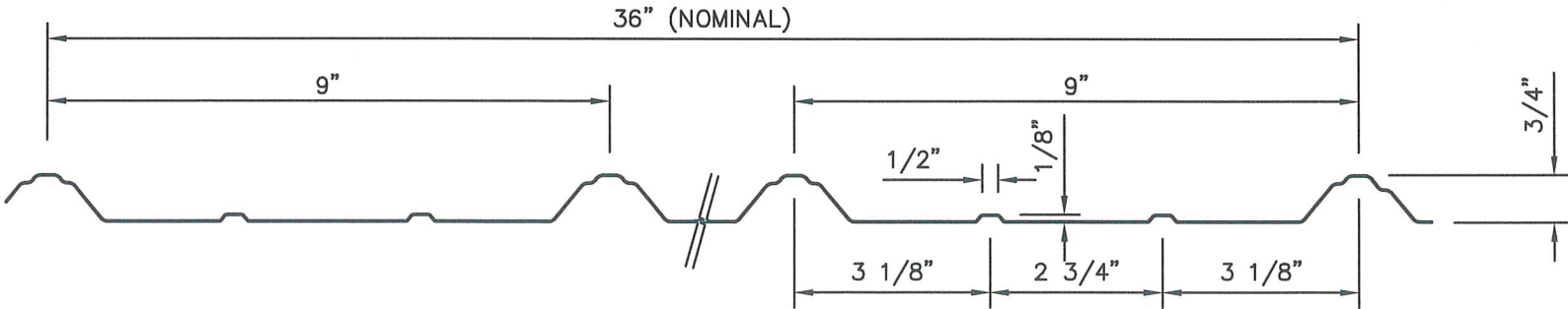
PANEL PROFILE
